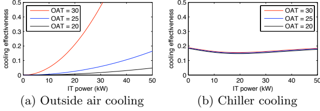
Figure 5: Cooling ineffectiveness comparison
