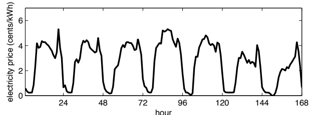
Figure 3: One week real-time electricity price
