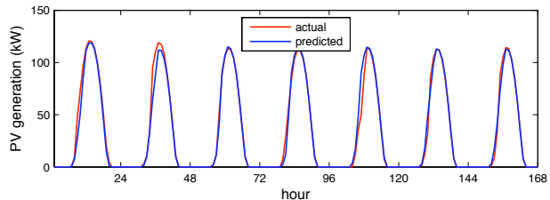
Figure 8: PV prediction
