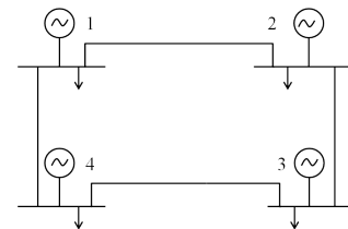
Fig. 1: A 4-area interconnected system
