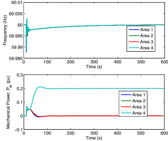
Fig. 2: The ACE-based AGC
